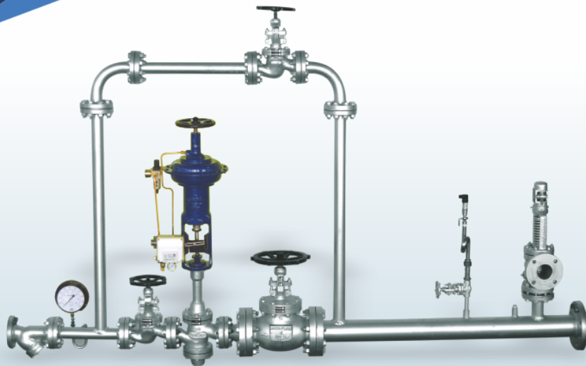
Pressure Reducing Station - Steam
